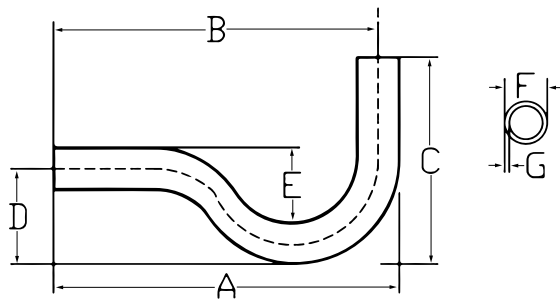
P Trap
