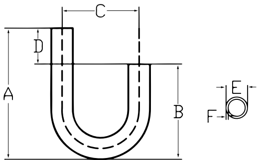
J Trap
